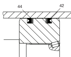
Lipseal Piston
