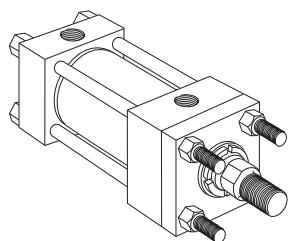
Style TB Tie Rods Extended Head End (NFFA Style MX3)
