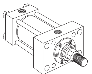
Style JJ Rectangular Head (NFA Style ME5)
