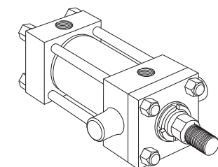
Style D Head Trunnion (NFPA Style MT1)
